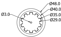
VISTA FRONTAL
