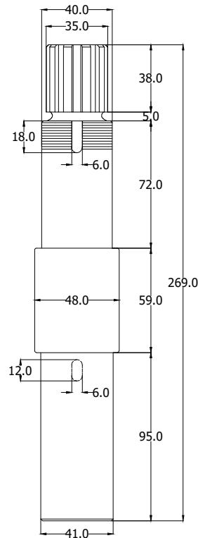
VISTA FRONTAL
